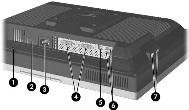
Rear Components
